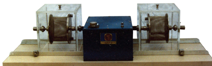
Slake Durability Apparatus
